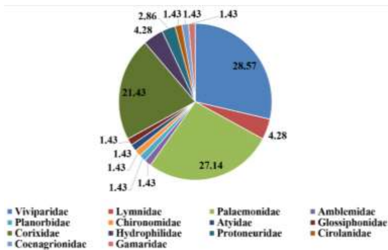
Fig. 3: Distribution of macro-invertebrate families at Digba Ghat in summer season
