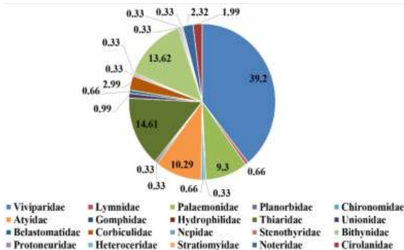
Fig. 9: Distribution of macro- invertebrate families at Fatuha in summer season
