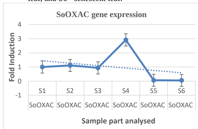
Fig. 2: SoOXAC gene expression in samples S1 to S6 of Amaranthus cruentus S1 - root, S2 - stem, S3 - mature leaf, S4 - young leaf, S5 - insect attacked leaf, and S6 - senescent leaf.
